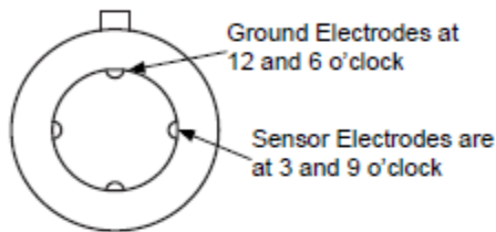
Meter/Sensor Orientation
