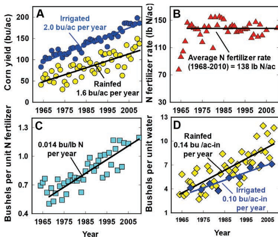
Figure B-2. Trends in corn grain yield (A), N fertilizer rate (B), grain yield produced per unit of N fertilizer ( NUE_r ) (C), and per unit of in-season water (WUE) (D) for the period from 1965-2010. Separate trends are shown for rainfed (yellow) and irrigated crops (blue) in (A) and (D). In-season (May-Aug.) water includes rainfall and irrigation. Rainfall data (D) were retrieved from five representative locations in Nebraska. Yield, N fertilizer, and irrigation water data were retrieved from USDA-NASS.
