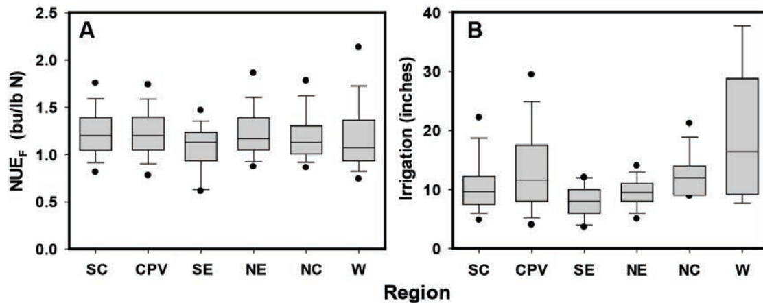
Figure B-4. Box plots for field N use efficiency (NUE F ) and total irrigation showing the variation across irrigated corn fields in the six regions in Nebraska for the 2009 crop season (SC: South Central; CPV: Central Platte Valley; SE: Southeast; NE: Northeast; NC: North Central; W: West).
