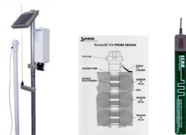
Figure J-8. Examples of the AquaSpy, EnviroSCAN, and ECHO capacitance probes for soil water monitoring.
